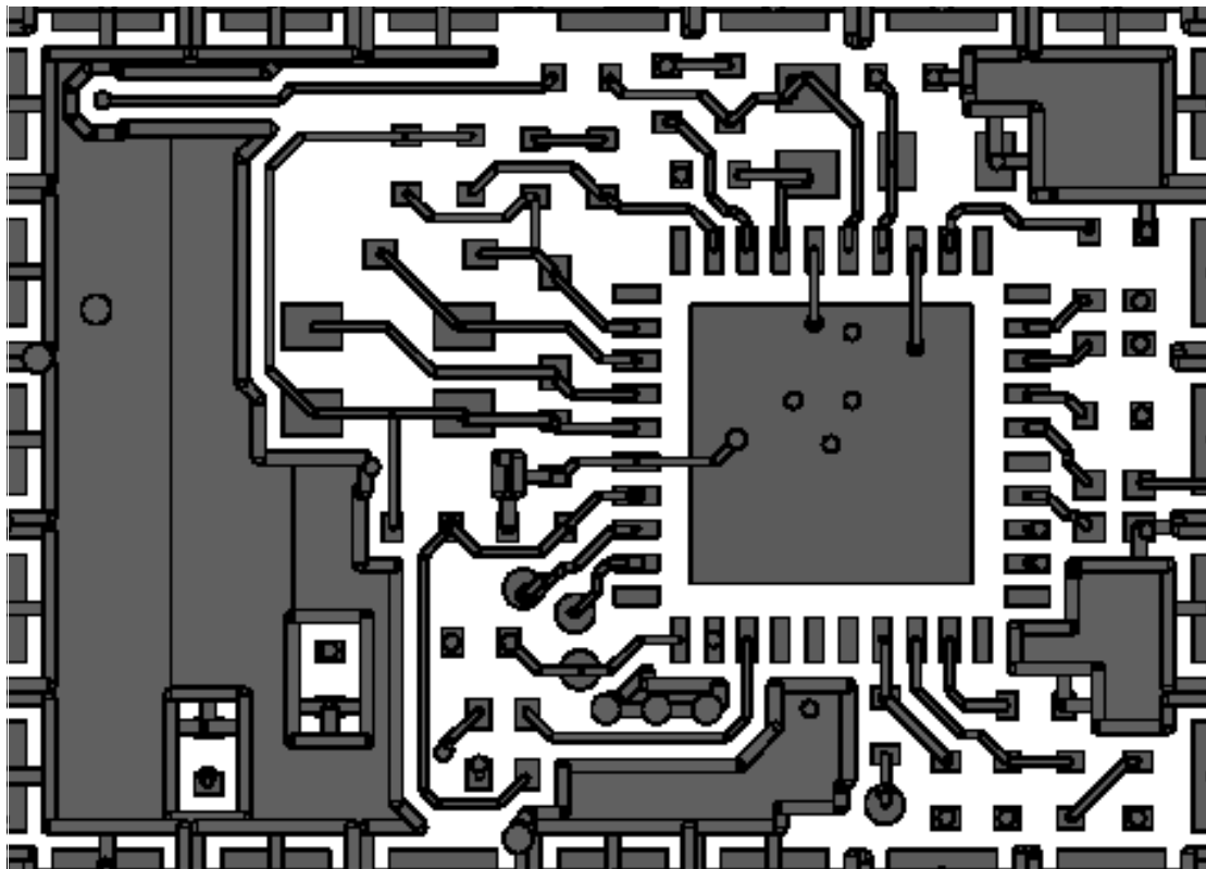
Figure 33: Trace layout.
