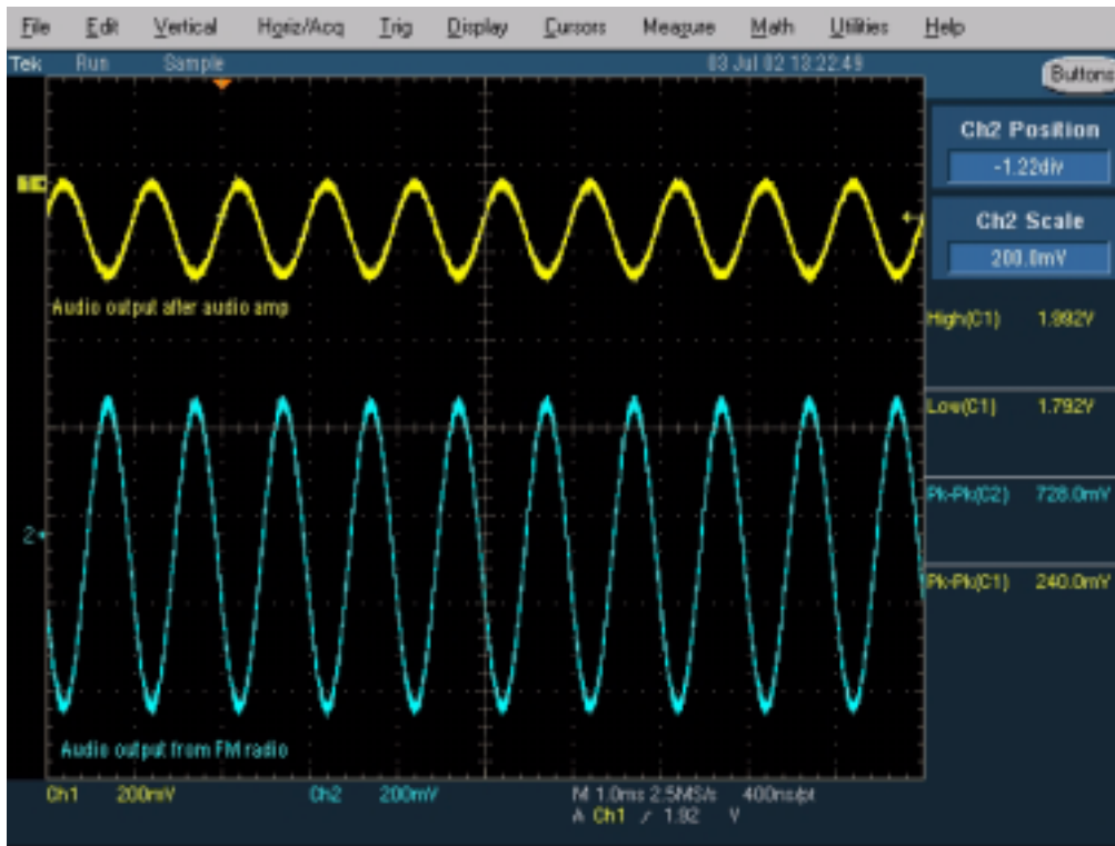
Figure 36: Oscilloscope screen shot, Audio output Signal 1: Audio output from PWB test points J103 and J104, with FM test signal, volume 100%. Signal 2: Audio output from FM radio pins 22 and 23(same as in C162 and C163), with FM test signal
