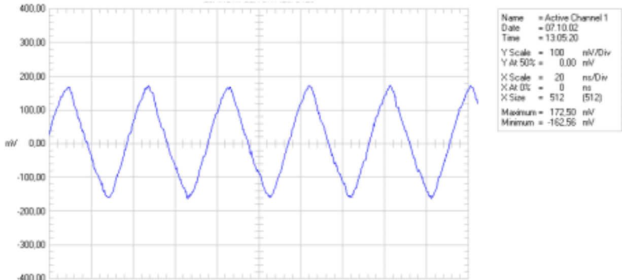
Figure 17: 1800 TX, channel 512, burst mode
