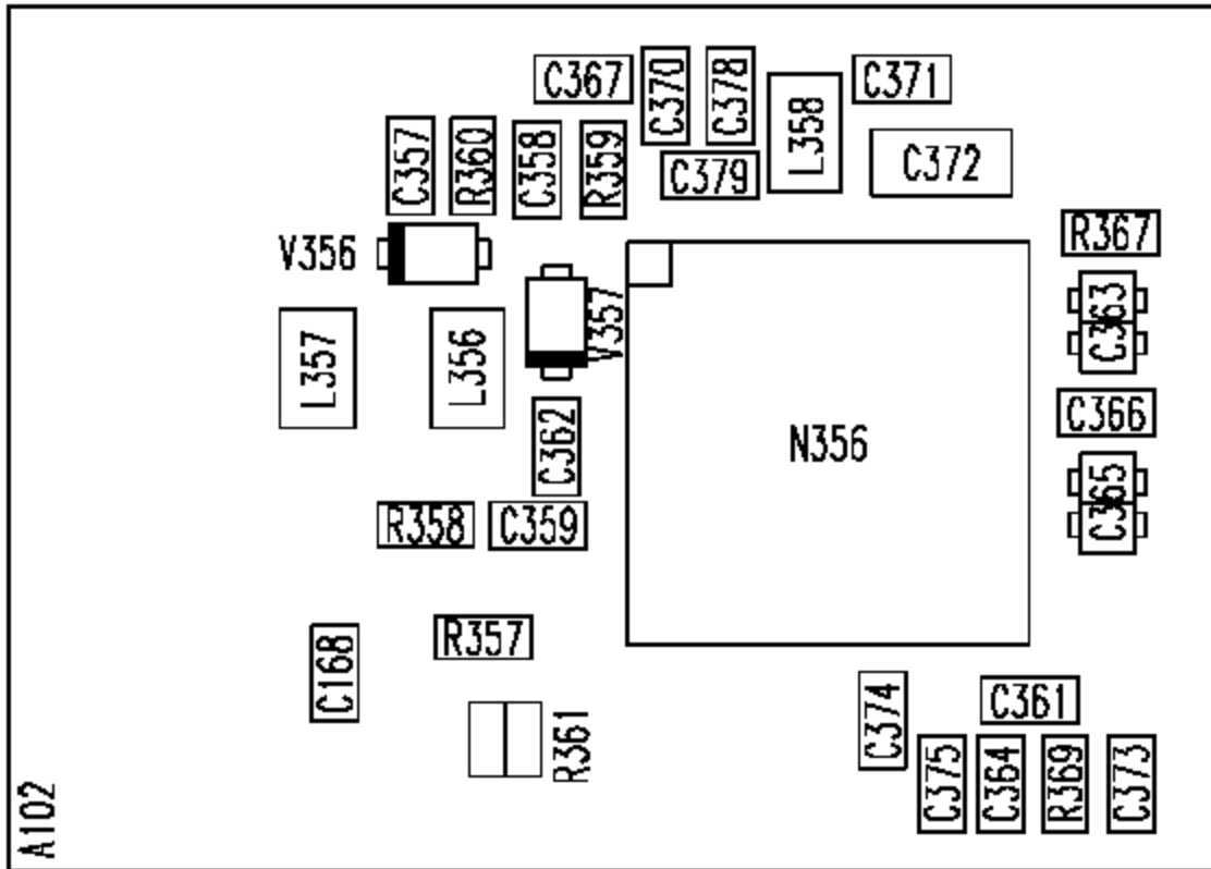
Figure 32: Component placement
