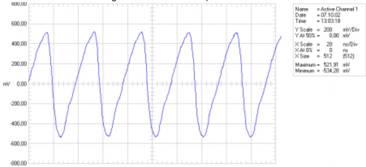
Figure 16: 26MHz RFCLK at R420/C420
