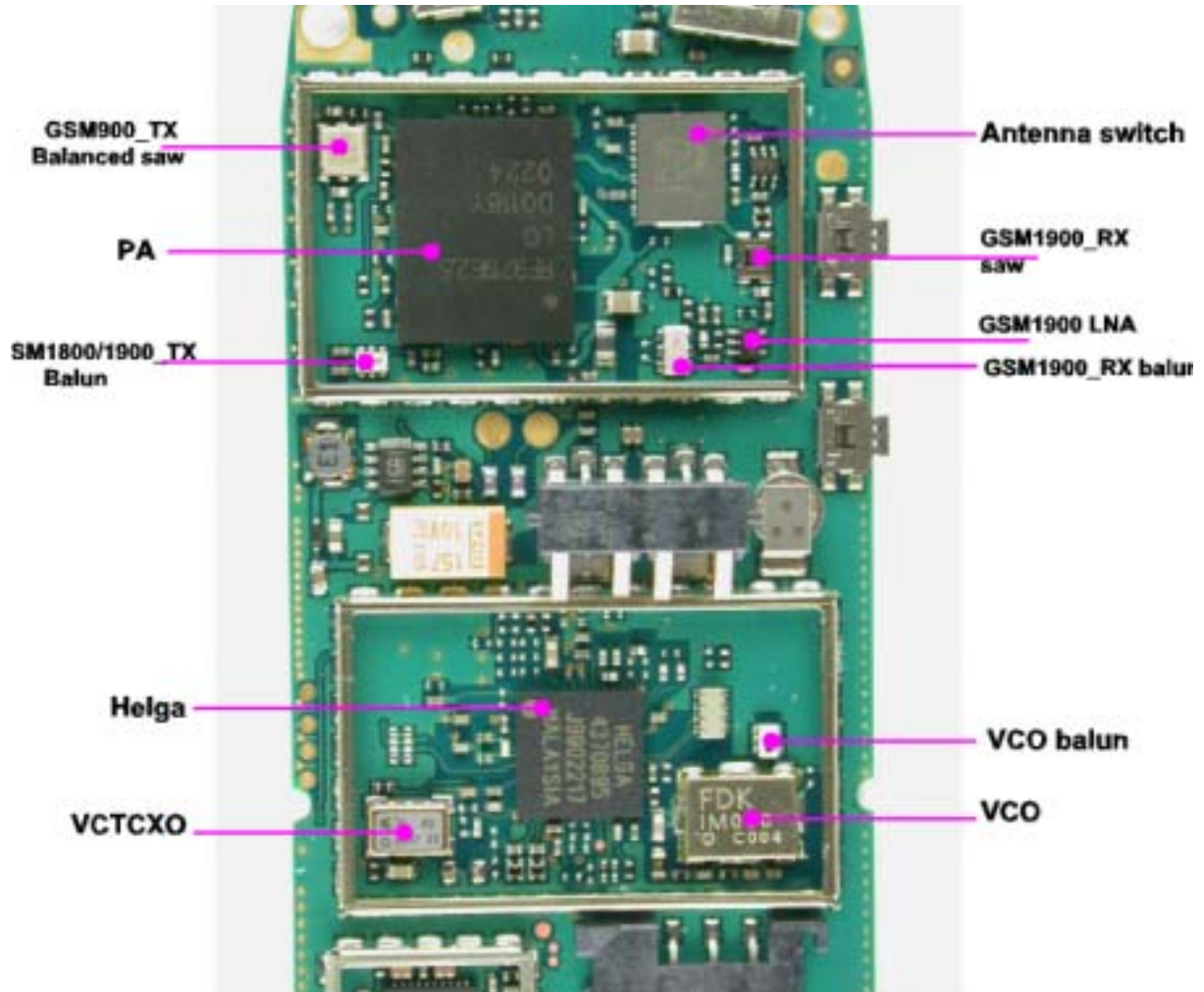
Figure 1: Component placement 1
