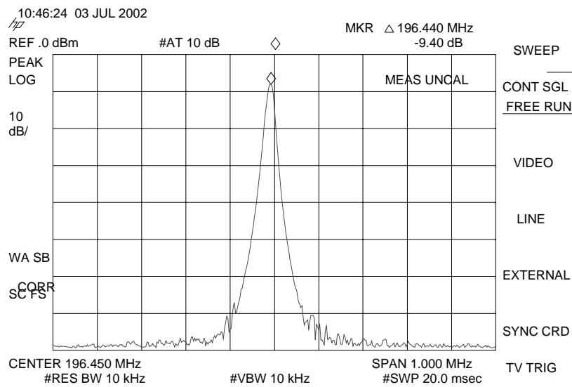
Figure 39: VCO frequency from FM radio pins 3 and 4, the other ends of V356 and V357, with FM test signal
