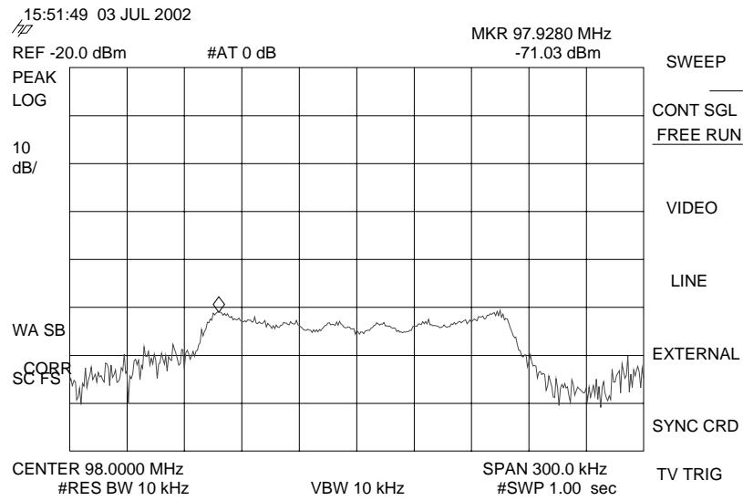
Figure 38: FM frequency from FM radio pin 37, the other end of L358, with FM test signal
